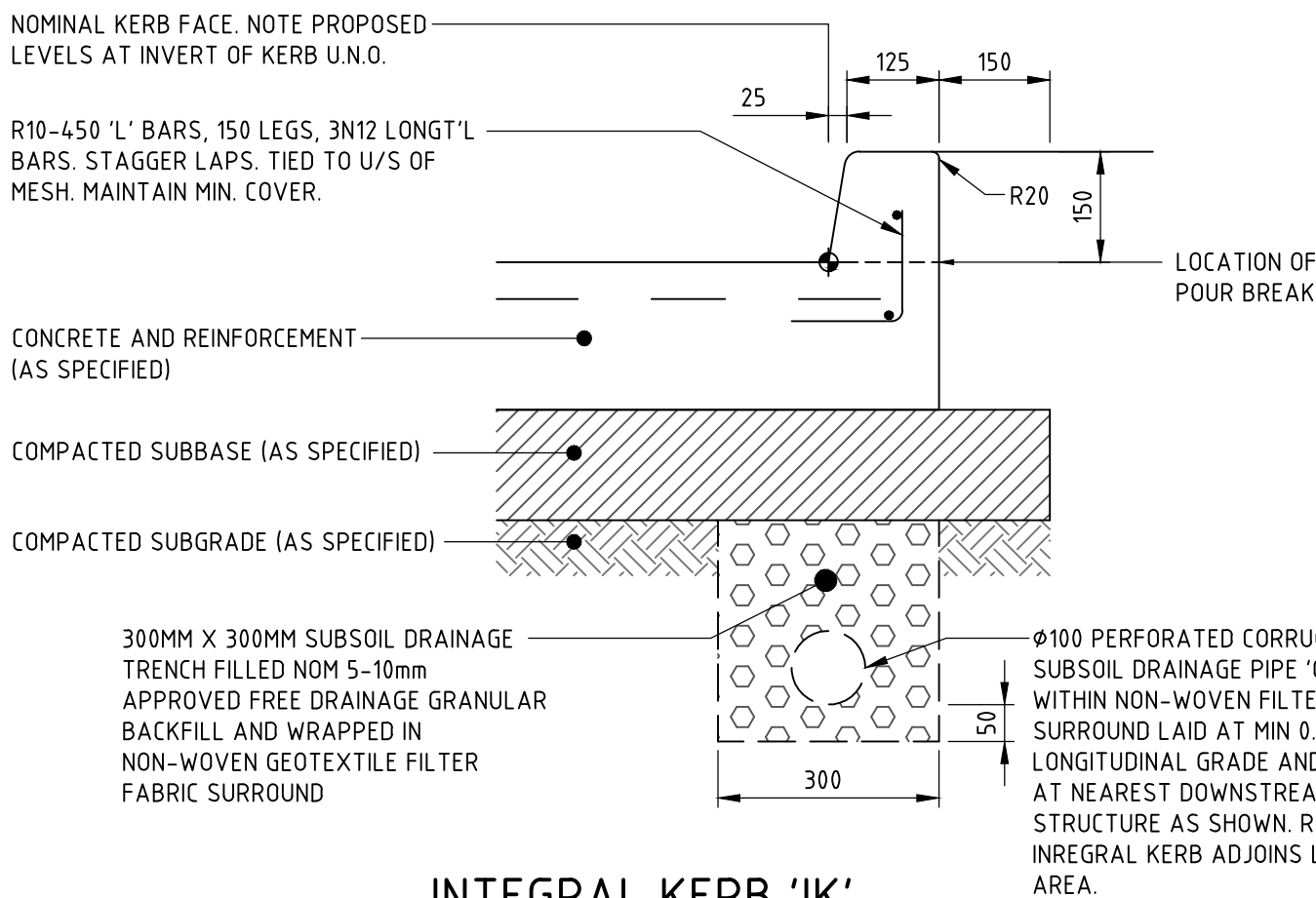
INTEGRAL KERB 'IK' PROVIDE TOOL JOINTS @ MAX 3m CENTRES AND TO MATCH SAWN AND DOWELED JOINTS. DISCONTINUE LONG'L REINF'T AT ALL JOINTS. ALL RADII'S TO BE 20mm UNLESS NOTED OTHERWISE
