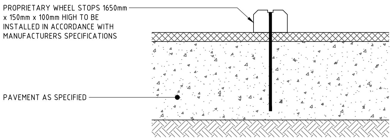
WHEEL STOP 'WS' WHEEL STOPS TO BE INSTALLED IN ACCORDANCE WITH AUSTRALIAN STANDARDS AS2890.1
