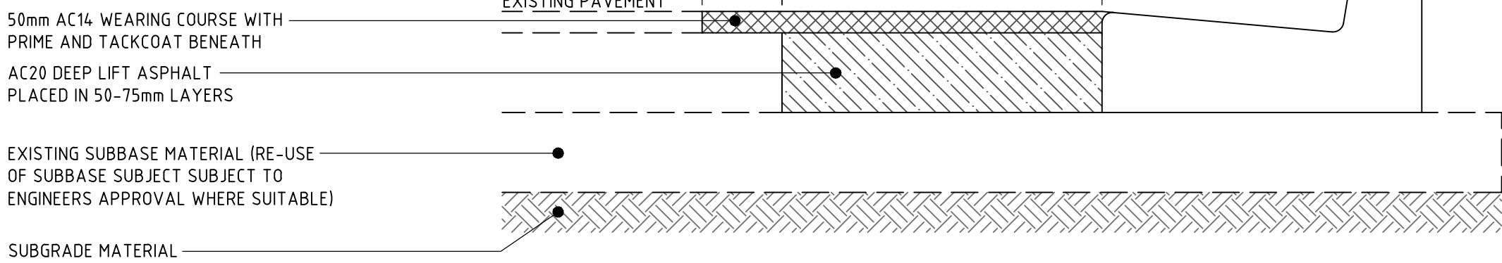
PAVEMENT INTERFACE 'INT1' MIN CBR ____% (CONTRACTOR TO CONFIRM ONSITE)
