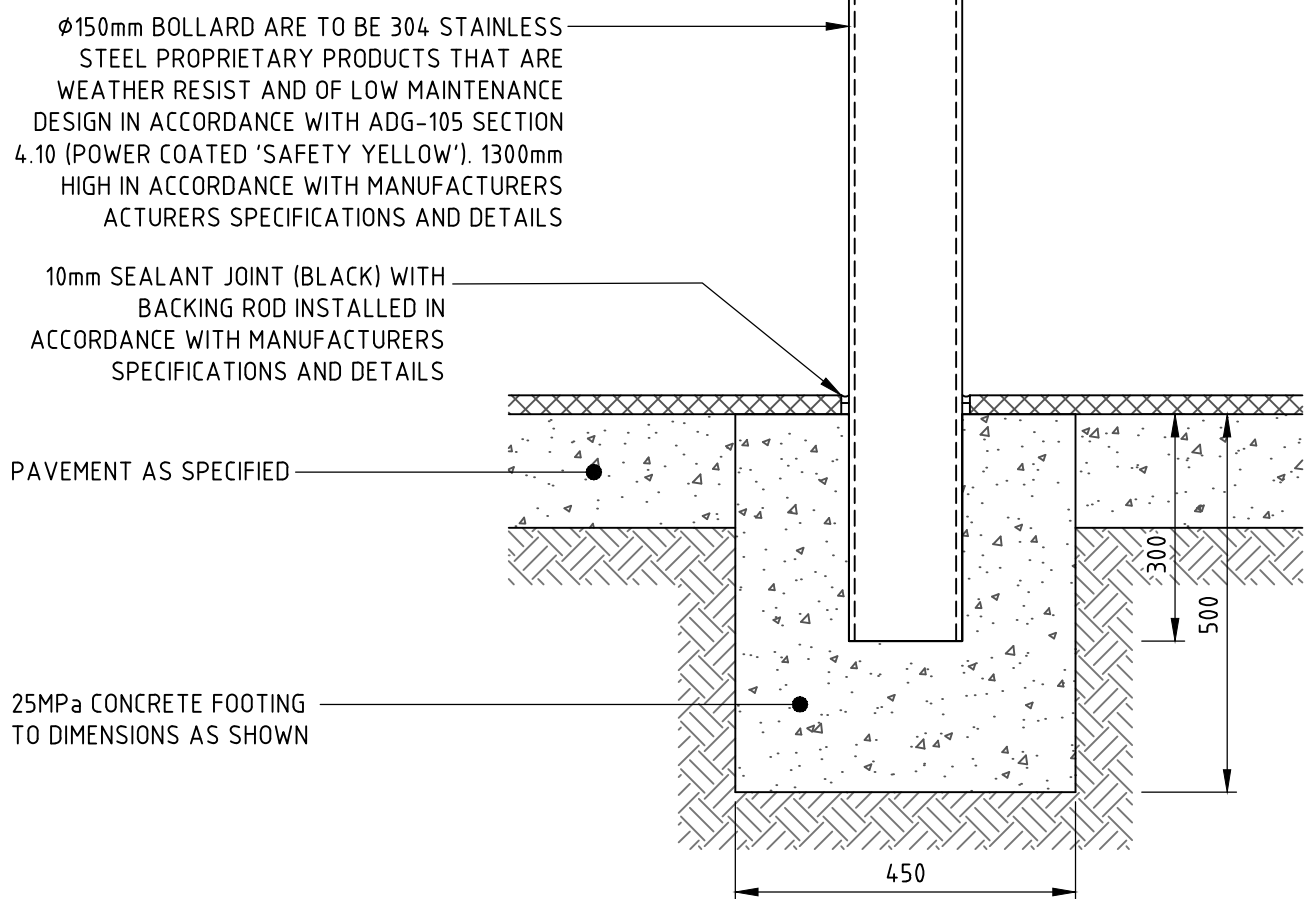
BOLLARD 'B' PROVIDE 600mm CLEARANCE TO FACE OF KERB / TRAVEL LANE
